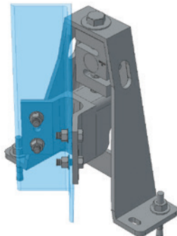
ANGLE IRON LEG ADAPTER
