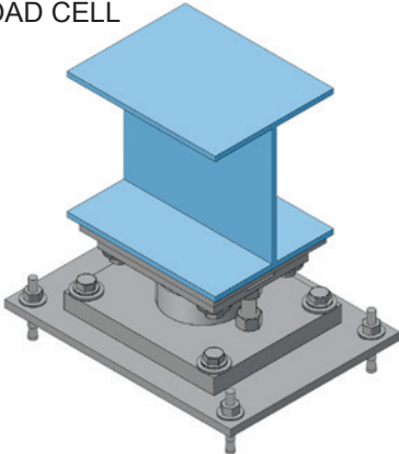
I-BEAM ON PANCAKE LOAD CELL
