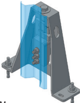
I-BEAM ON PANCAKE LOAD CELL
